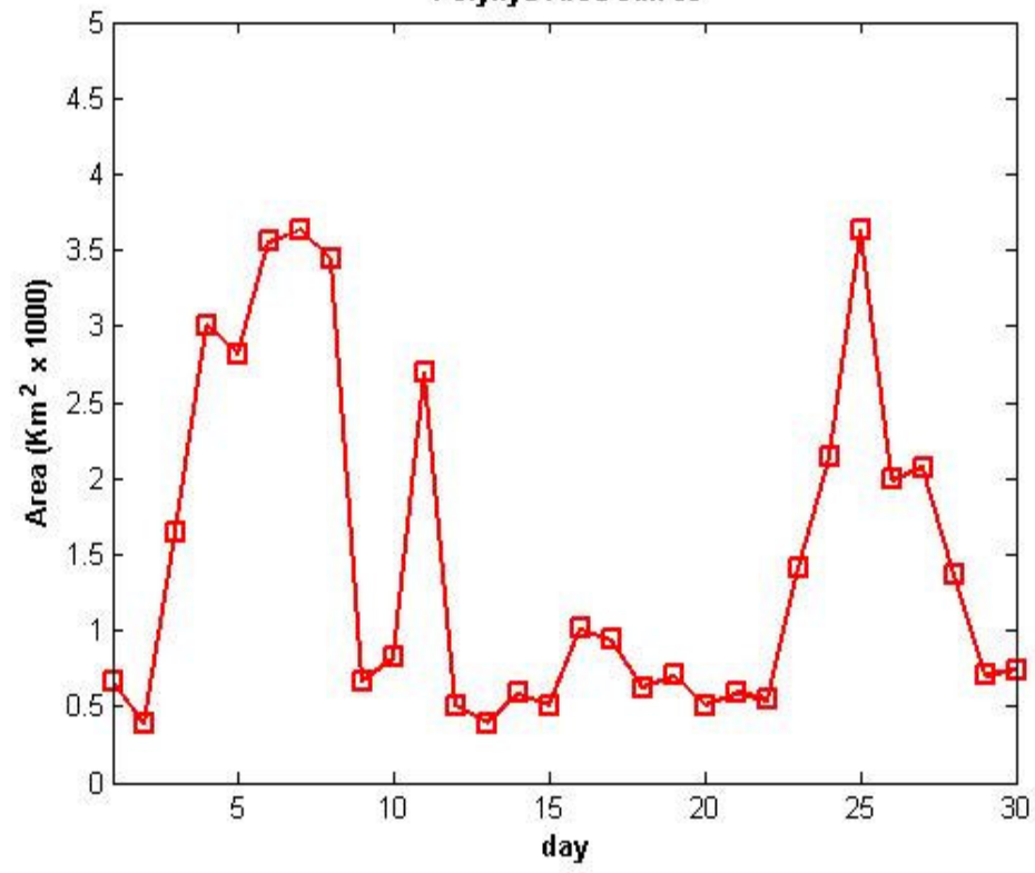
Polynya Area Jun 06
