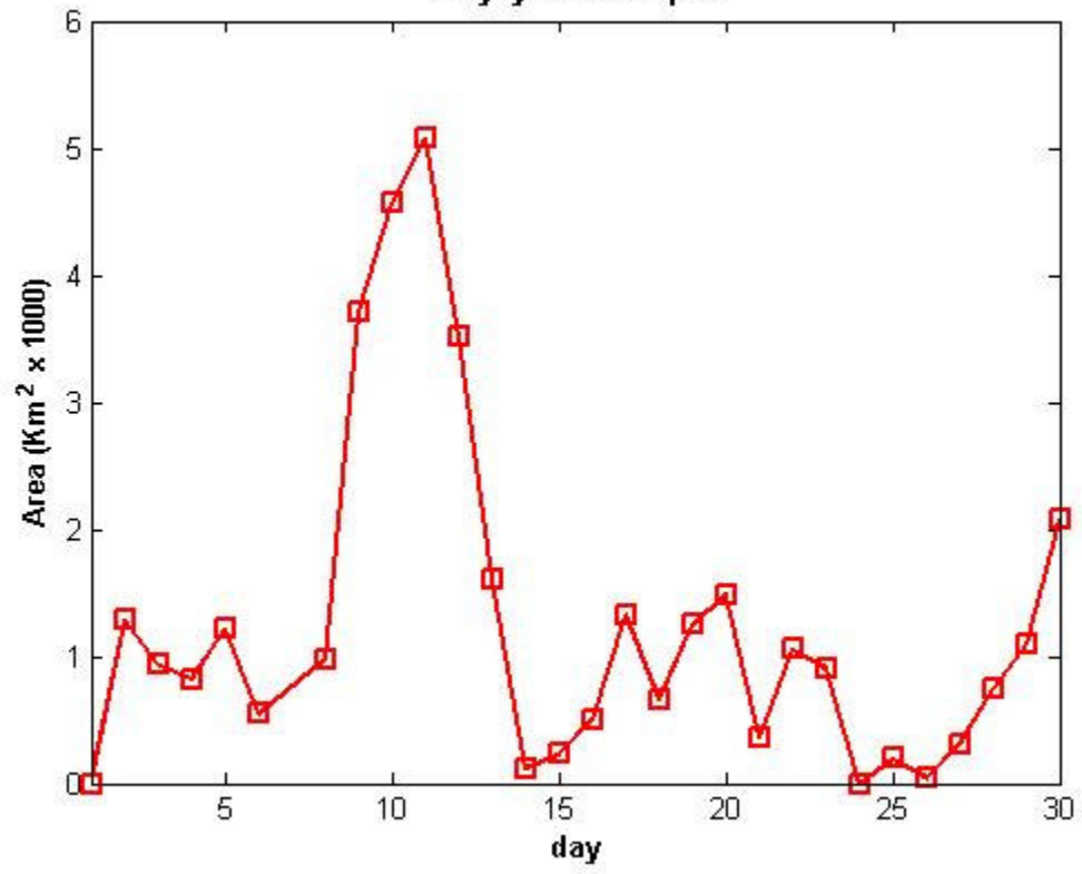
Polynya Area Sep 06
