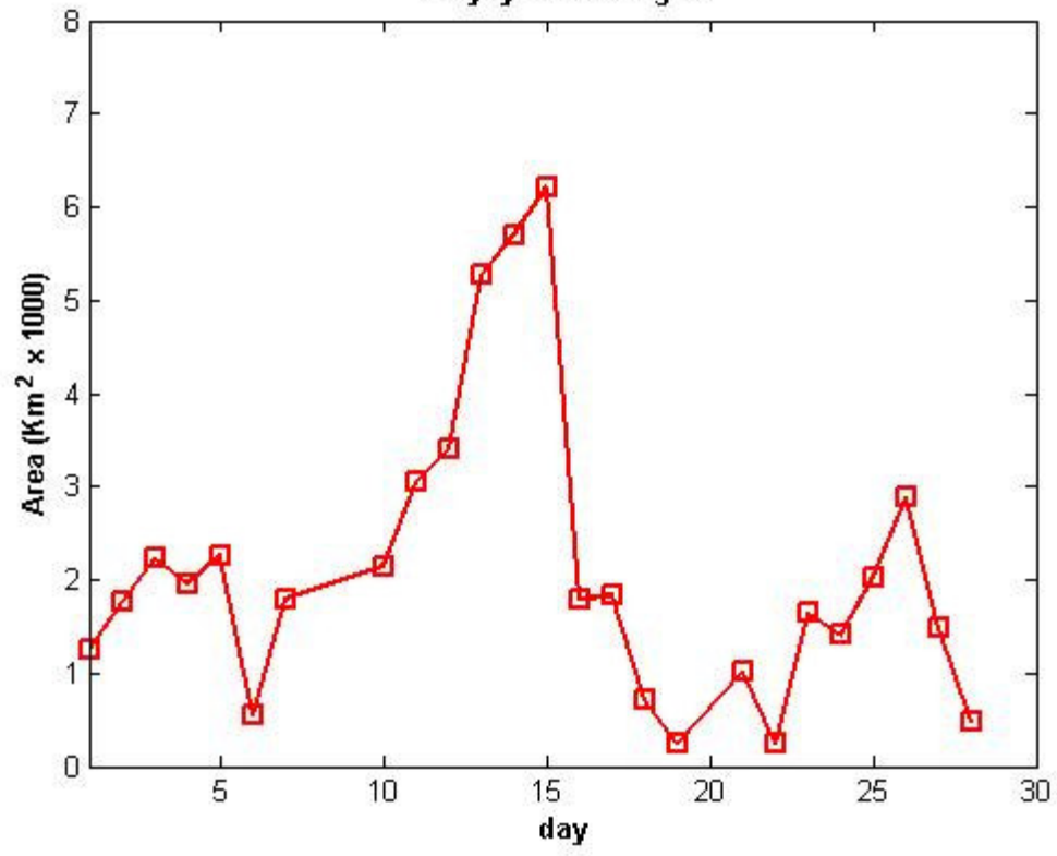
Polynya Area Aug 06
